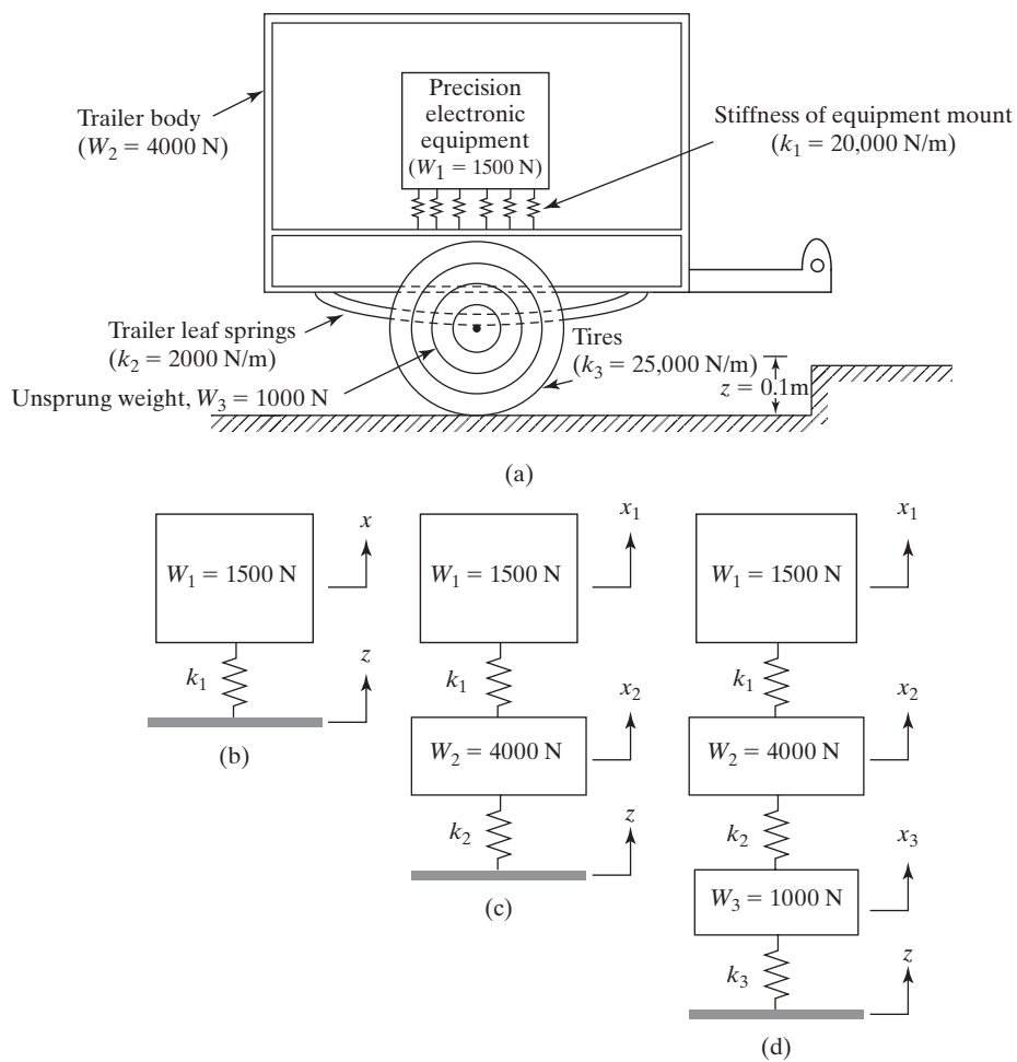
FIGURE 6.45 Three models of a trailer-carrying electronic equipment.
