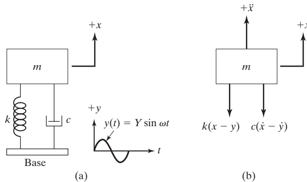
FIGURE 3.14 Base excitation.
