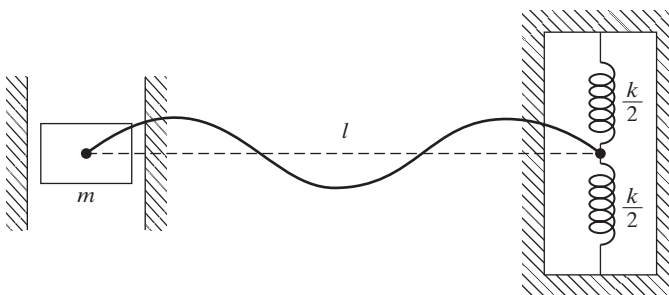
FIGURE 8.24 Cable connected to mass at one end and springs at the other end.
