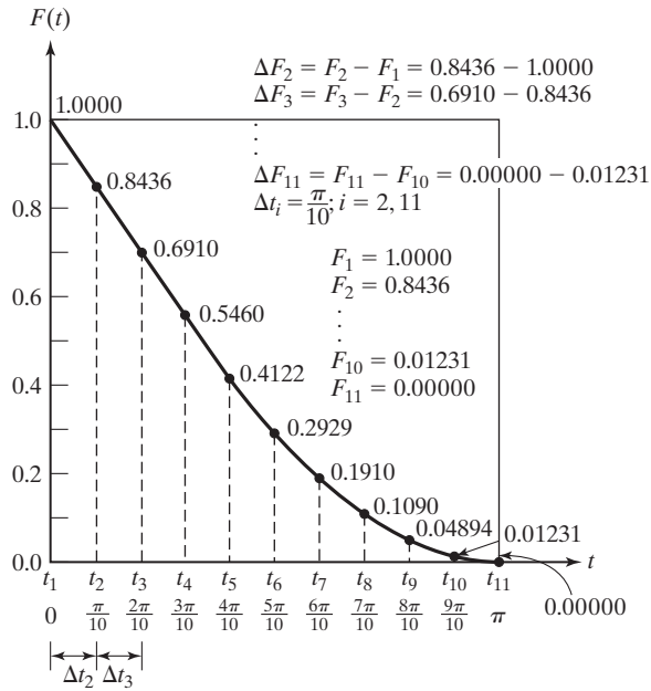
FIGURE 4.36 Piecewise linear approximation.
