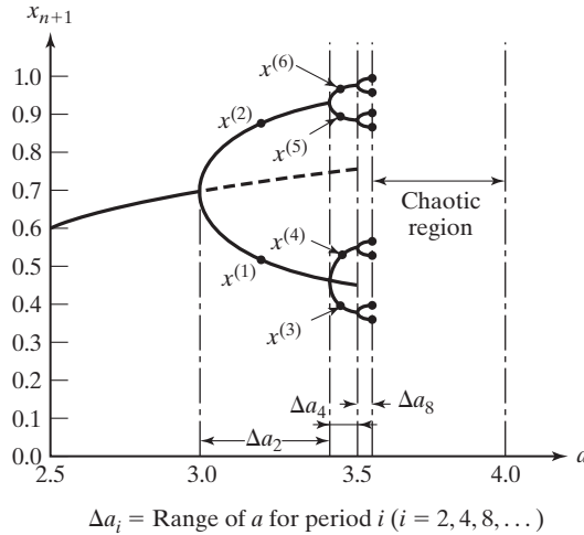
FIGURE 13.20 Bifurcation plot.
