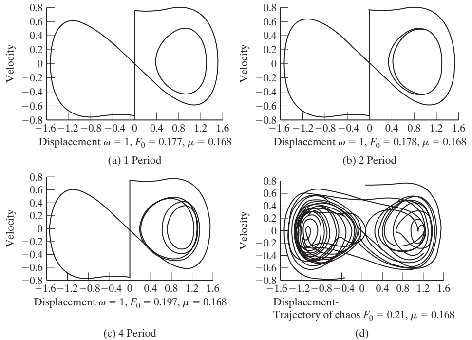
FIGURE 13.26 Distortion of phase plane. (From [13.33]; reprinted with permission of American Society of Mechanical Engineers.)
