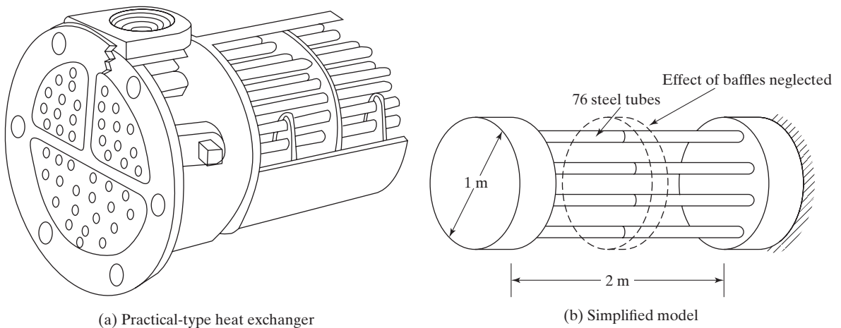
FIGURE 1.125 Shell-and-tube exchanger.
