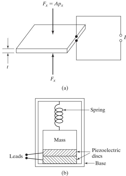
FIGURE 10.5 Piezoelectric accelerometer.
