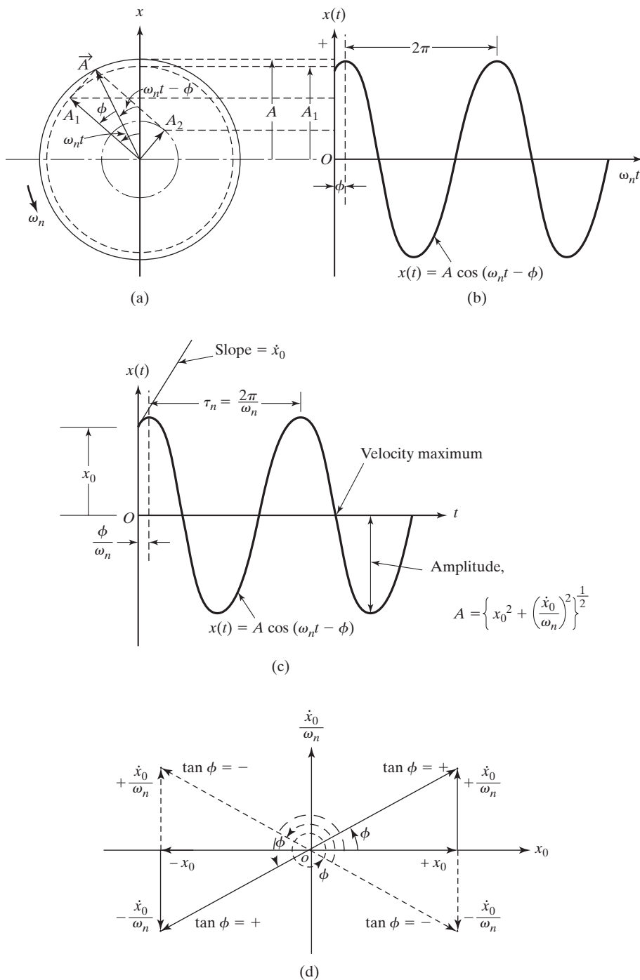
FIGURE 2.8 Graphical representation of the motion of a harmonic oscillator.
