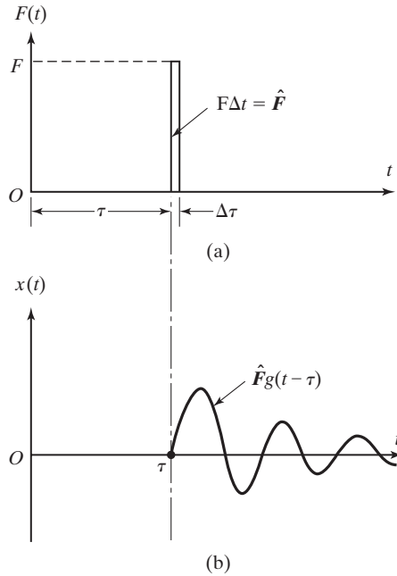
FIGURE 4.7 Impulse response.
