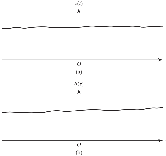
FIGURE 14.6 Constant values of function.
