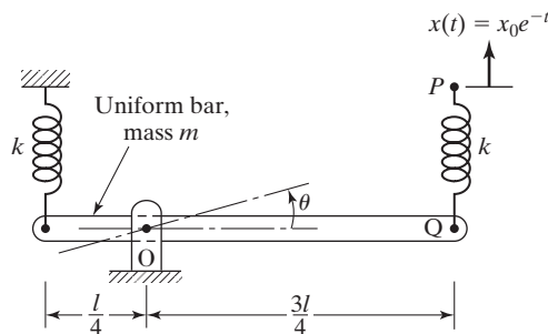
FIGURE 4.55 Rigid bar undergoing rotational motion.
