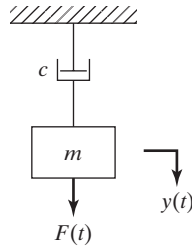
FIGURE 14.30 Mass-damper system subjected to force F(t) .
