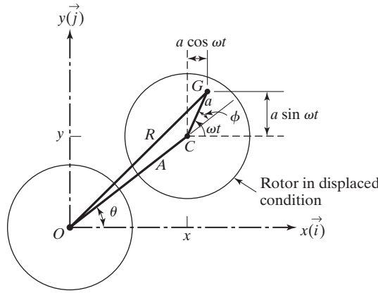
FIGURE 9.12 Rotor with eccentricity.
