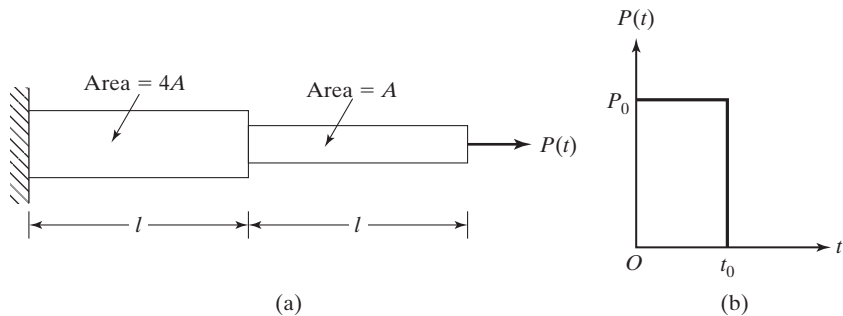
FIGURE 12.37 Stepped bar with end load.
