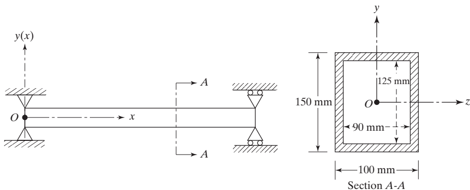
FIGURE 7.16 Beam with hollow rectangular section.
