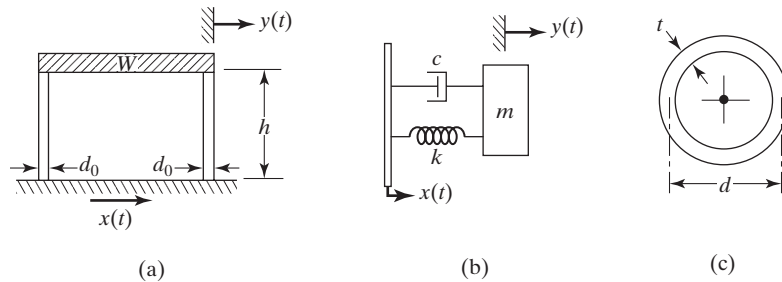
FIGURE 14.21 Single-story building.
