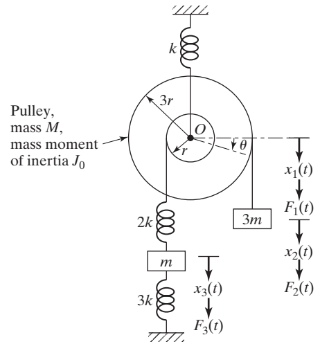
FIGURE 6.21 Pulley attached to springs and masses.
