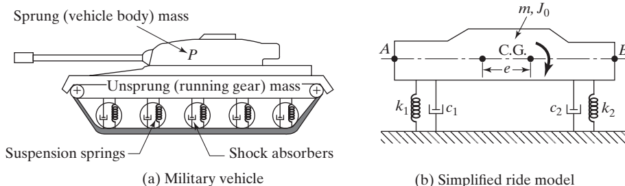
FIGURE 5.40 Military vehicle.
