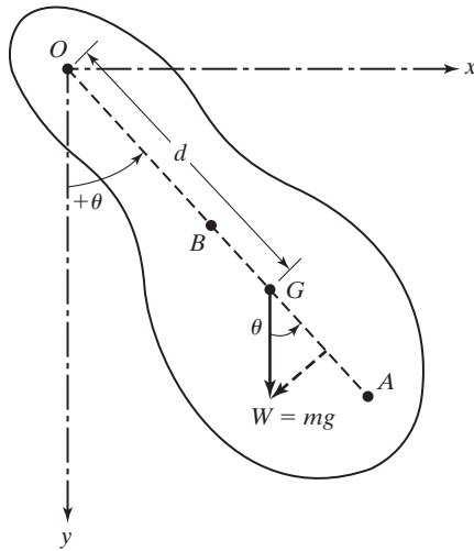
FIGURE 2.15 Compound pendulum.
