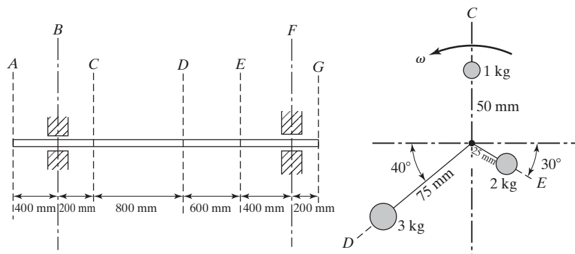
FIGURE 9.45 Shaft with unbalanced masses.
