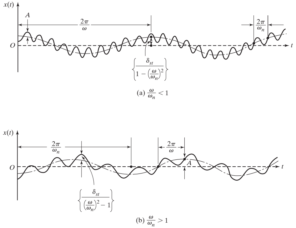
FIGURE 3.7 Total response.
