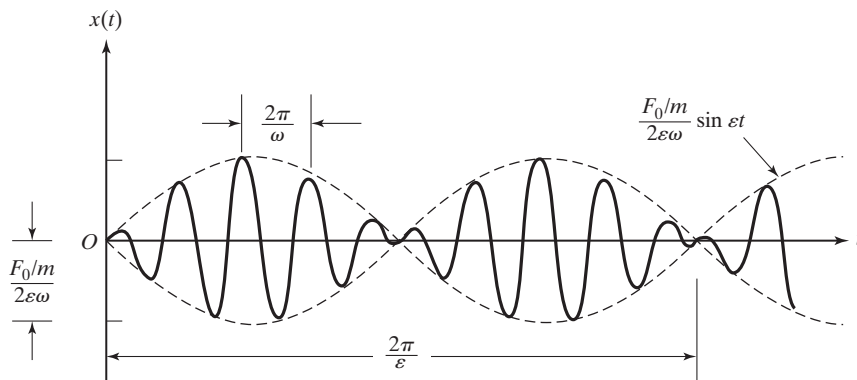
FIGURE 3.8 Phenomenon of beats.
