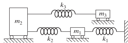
FIGURE 6.32 Three-degree-of-freedom spring-mass system.
