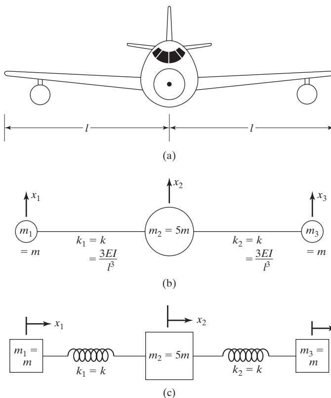
FIGURE 6.26 Airplane in vertical motion.
