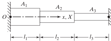
FIGURE 12.39 Fixed-fixed three-stepped bar.
