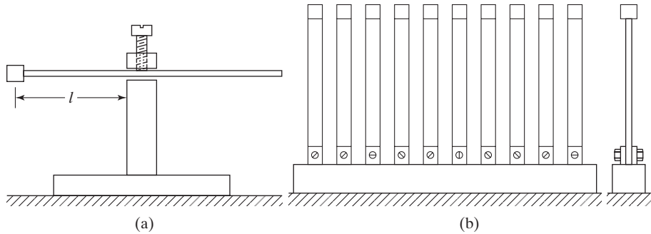
FIGURE 10.15 Frequency-measuring instruments.
