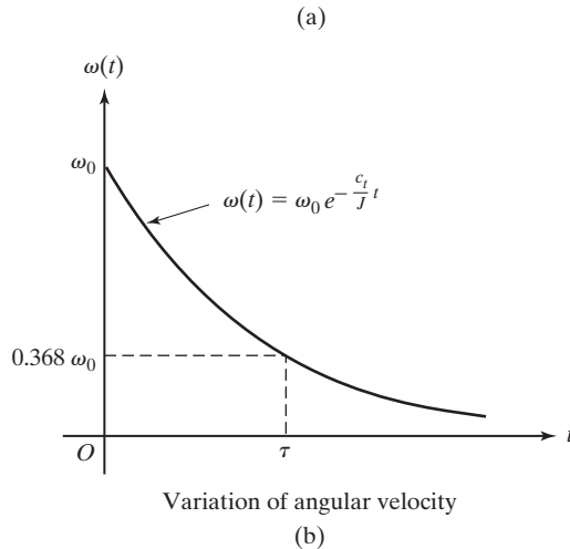
FIGURE 2.17 Rotor mounted in bearings and its angular velocity variation.
