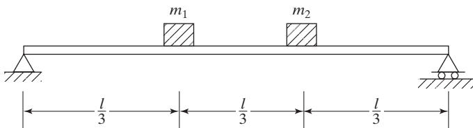
FIGURE 7.12 Simply supported beam carrying two masses.
