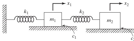
FIGURE 6.25 Damped two-degree-of-freedom system.
