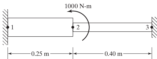
FIGURE 12.23 Stepped beam.
