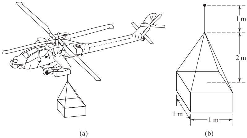
FIGURE 2.74 Crate hanging from a helicopter.
