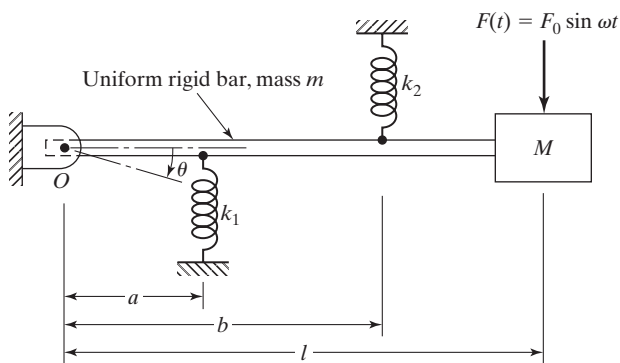
FIGURE 3.44 Spring-supported rigid bar subjected to harmonic force.
