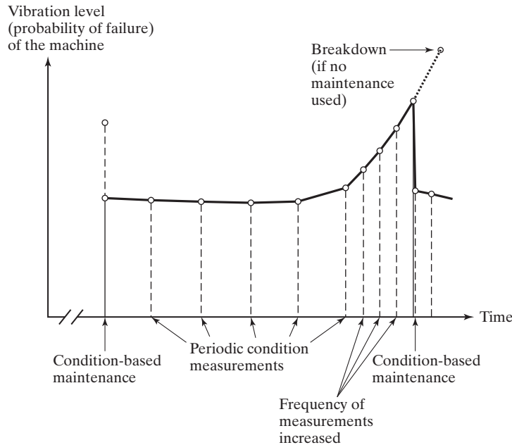
FIGURE 10.35 Condition-based maintenance.
