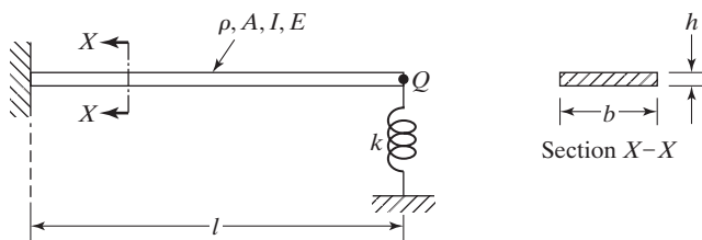
FIGURE 12.22 Cantilever beam with spring support at free end.
