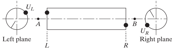
FIGURE 9.9 Two-plane balancing.
