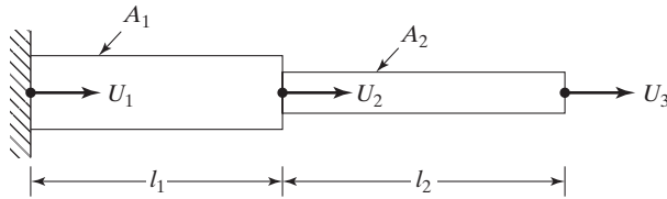
FIGURE 12.38 Stepped bar.
