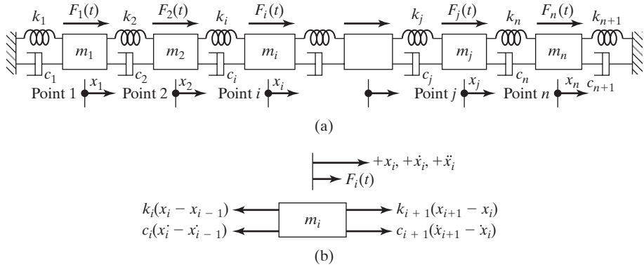
FIGURE 6.3 Spring-mass-damper system.
