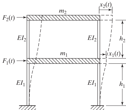
FIGURE 5.32 Two-story building frame.
