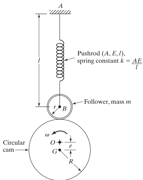
FIGURE 3.43 Cam-follower system.
