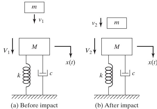
FIGURE 4.26 Elastic impact.
