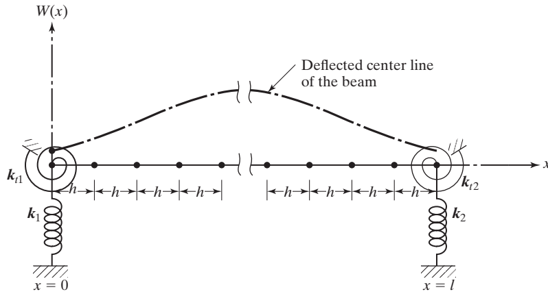
FIGURE 11.11 Elastically restrained beam.
