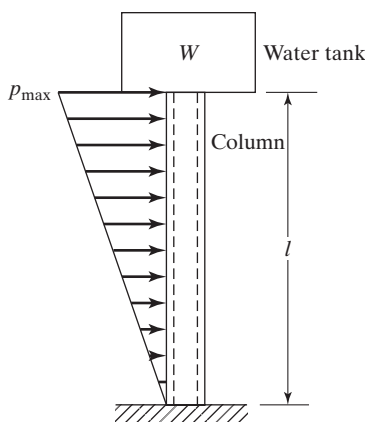
FIGURE 12.28 Water tank.
