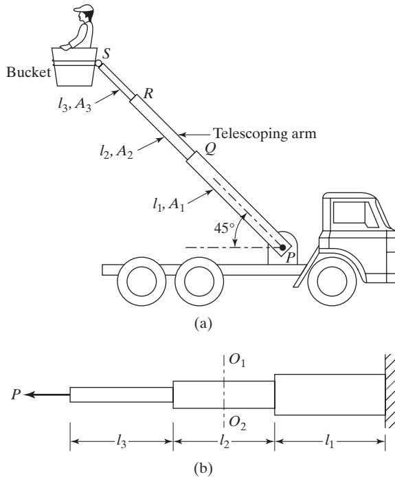
FIGURE 2.12 Telescoping boom of a fire truck.
