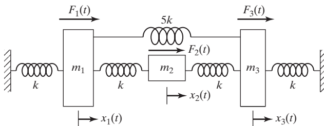
FIGURE 6.18 Three-degree-of-freedom spring-mass system.
