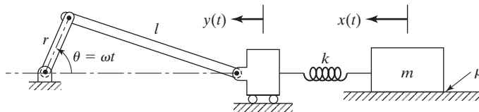
FIGURE 4.40 Base motion through slider crank mechanism.
