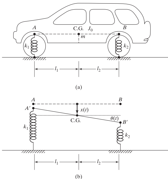
FIGURE 5.2 Car.
