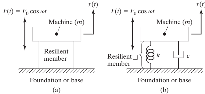
FIGURE 9.20 Machine and resilient member on rigid foundation.
