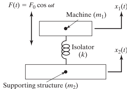
FIGURE 9.29 Machine with isolator on a flexible foundation.
