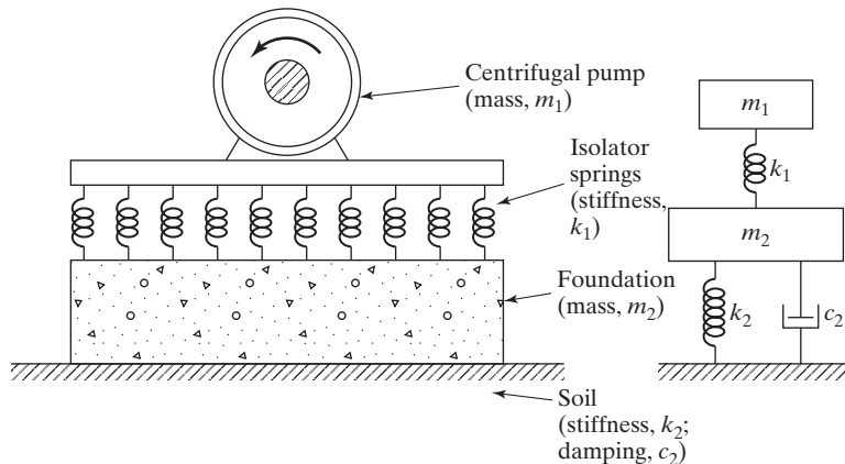
FIGURE 5.54 Centrifugal pump.
