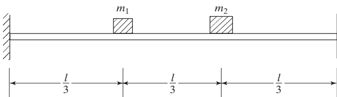
FIGURE 7.13 Fixed-fixed beam carrying two masses.
