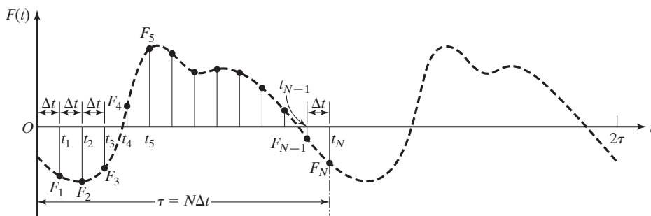
FIGURE 4.5 An irregular forcing function.
