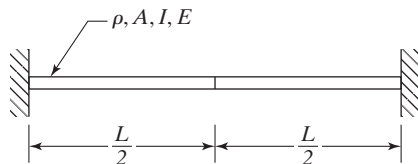
FIGURE 12.31 Fixed-fixed beam.
