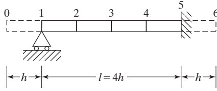
FIGURE 11.7 Simply supported-fixed beam.
