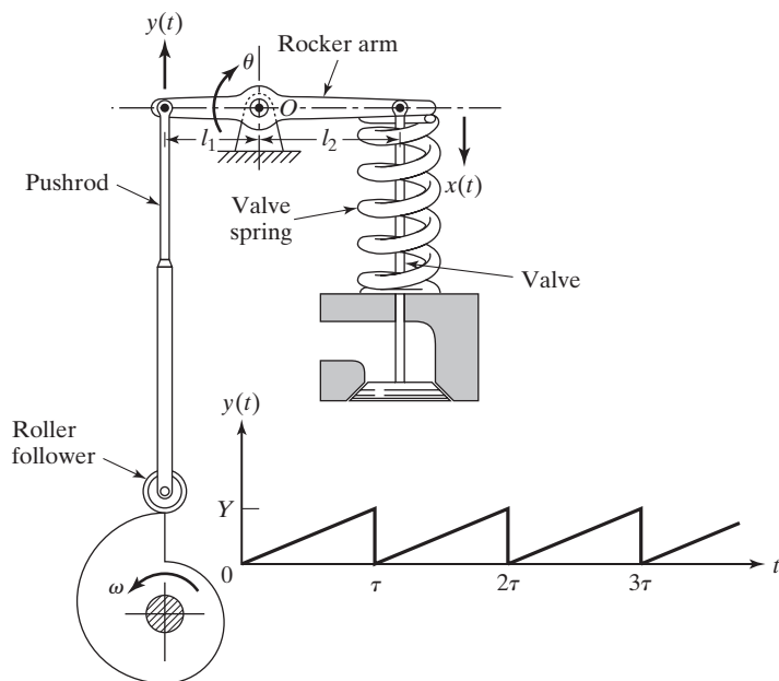
FIGURE 1.61 Cam-follower system.
