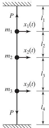
FIGURE 6.33 Tight string carrying three masses.
