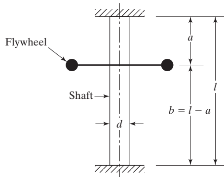
FIGURE 2.76 Flywheel mounted on a shaft.
