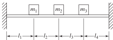
FIGURE 6.31 Fixed-fixed beam carrying three masses.
