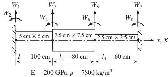
FIGURE 12.12 Stepped beam.
