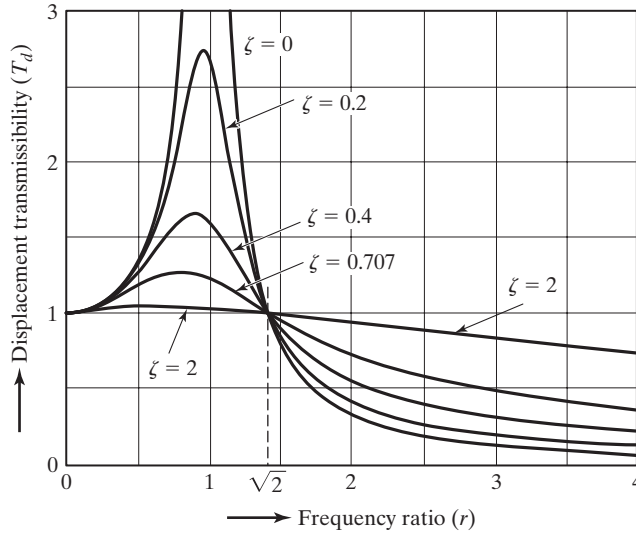
FIGURE 9.25 Variation of T_d with r (for base motion).
