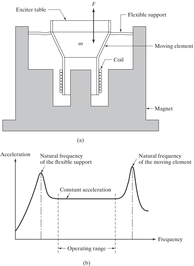
FIGURE 10.19 (a) Electrodynamic shaker. (b) Typical resonance characteristics of an electrodynamic exciter.
