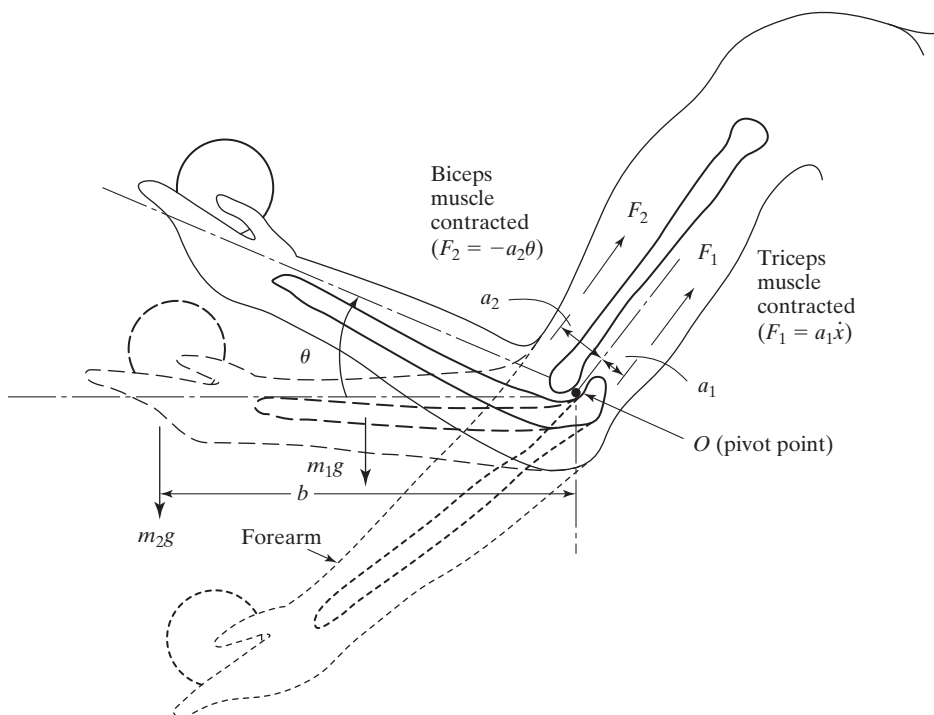
FIGURE 2.108 Motion of arm.
