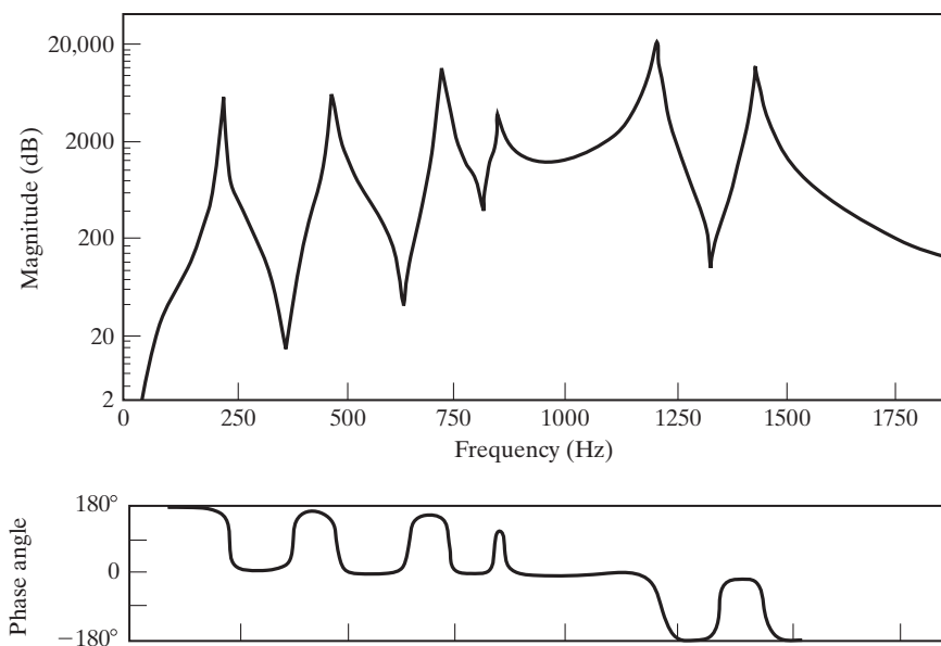
FIGURE 10.46 Experimental transfer function of structure.
