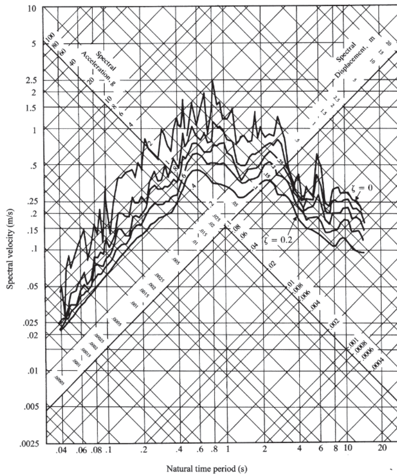
FIGURE 4.18 Response spectrum of a typical earthquake [4.12]. (Imperial Valley Earthquake, May 18, 1940; \zeta = 0, 0.02, 0.05, 0.10, \text{ and } 0.20 .) (Adapted with permission from The Shock and Vibration Digest .)
