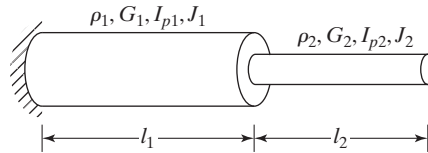
FIGURE 12.36 Stepped shaft.
