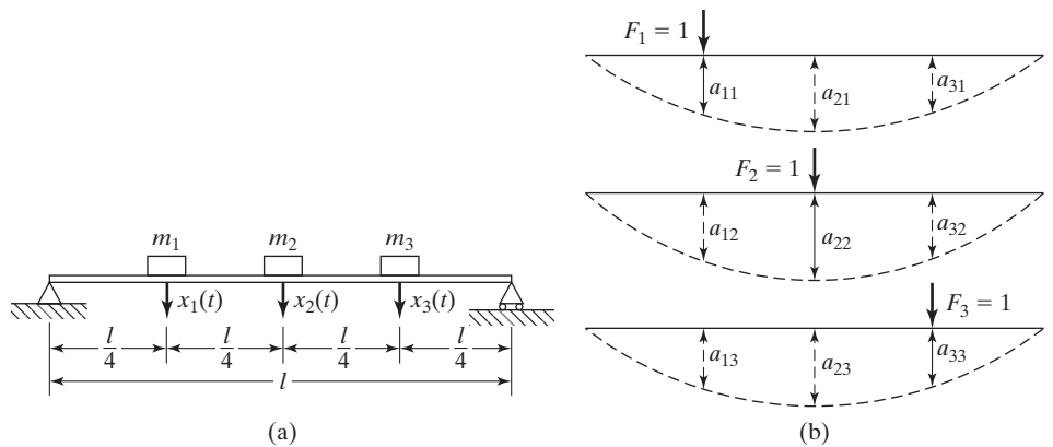
FIGURE 6.9 Beam deflections.
