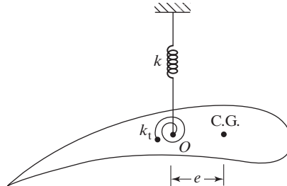
FIGURE 5.43 Airfoil.
