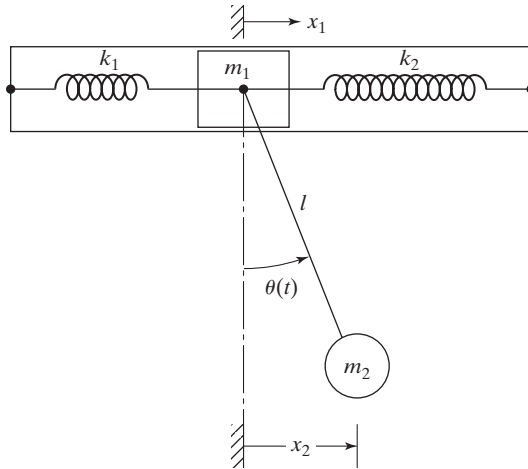
FIGURE 5.23 Piston-pendulum motions.
