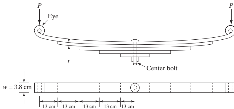
FIGURE 12.17 A multiple-leaf spring.
