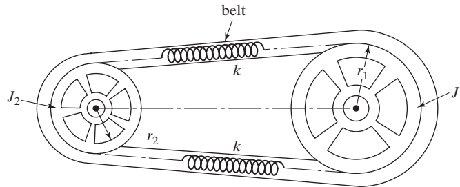
FIGURE 5.62 Two pulleys connected by belt.
