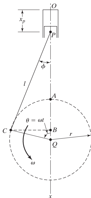
FIGURE 1.120 A slider crank mechanism.
