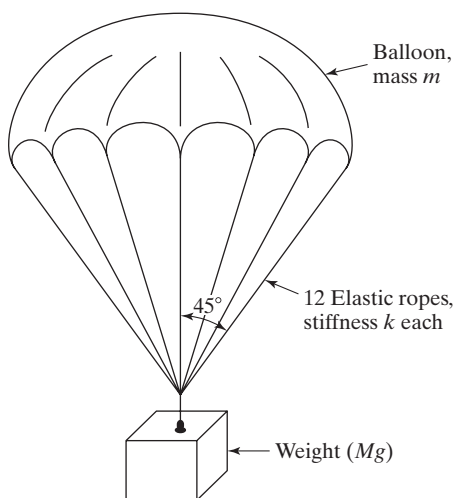
FIGURE 5.60 Hot-air balloon connected to a mass.
