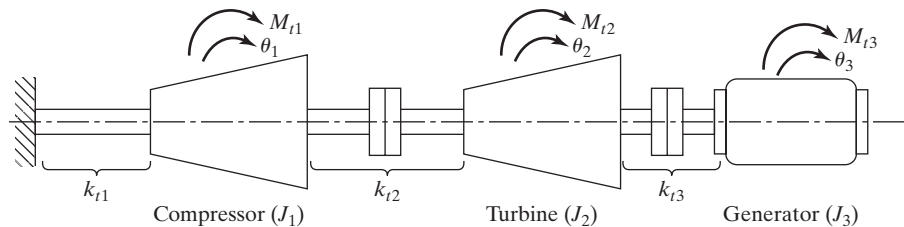
FIGURE 6.11 Torsional system.
