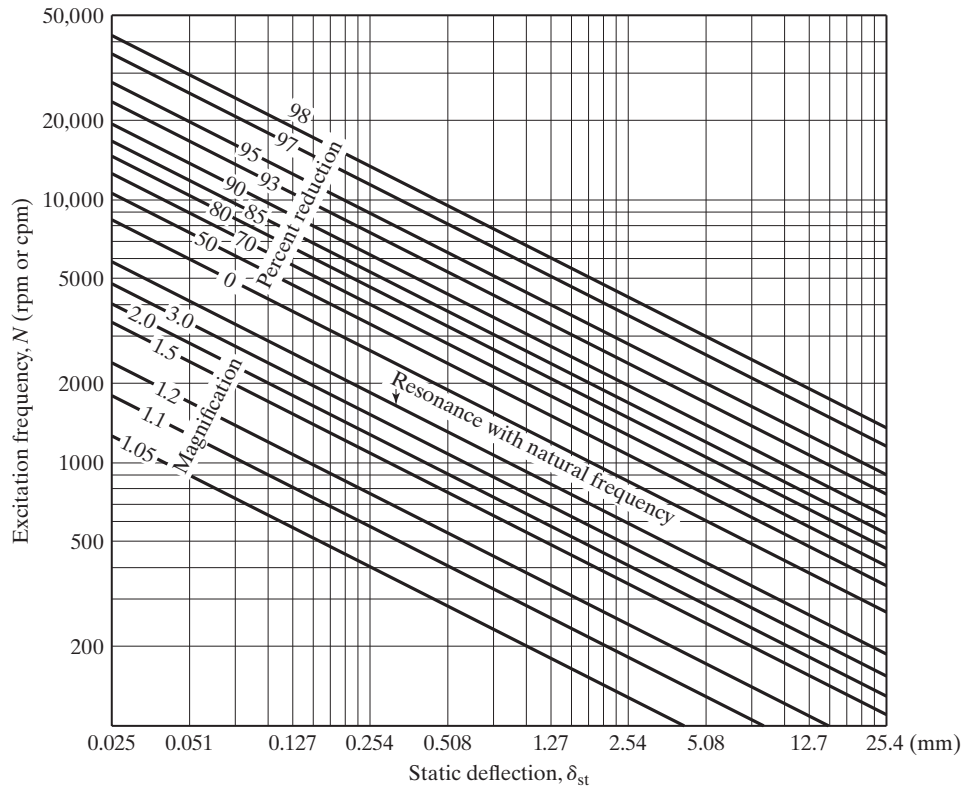
FIGURE 9.23 Isolation efficiency.
