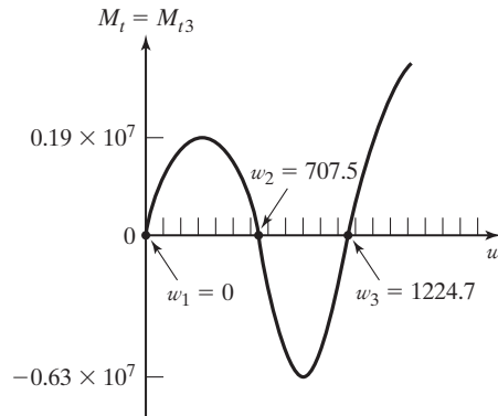
FIGURE 7.6 Resultant torque versus frequency.
