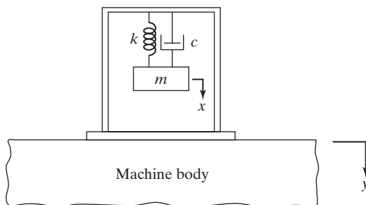
FIGURE 10.43 Motion of suspended mass relative to machine body.
