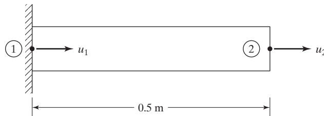
FIGURE 12.7 Uniform bar with two degrees of freedom.
