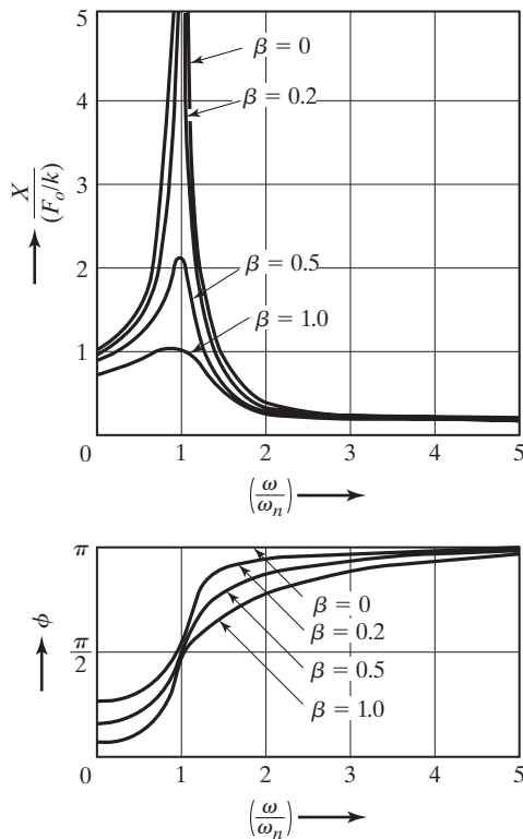
FIGURE 3.25 Steady-state response.
