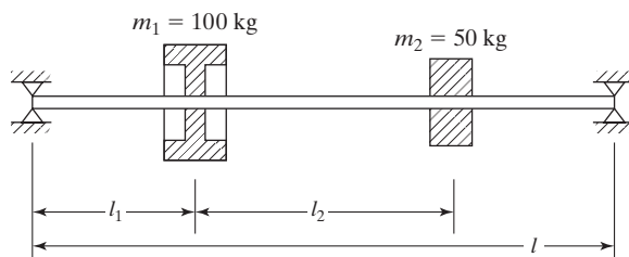
FIGURE 7.19 Shaft carrying flywheel and pulley.
