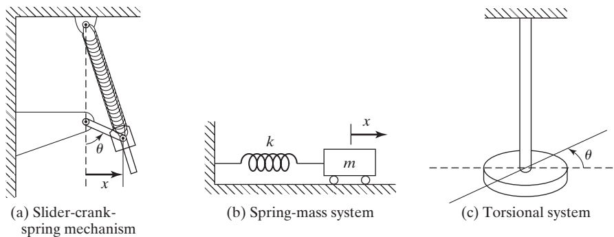
FIGURE 1.11 Single-degree-of-freedom systems.
