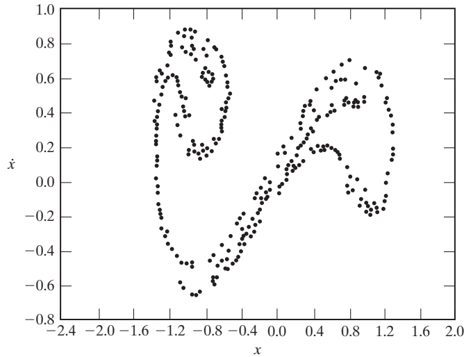
FIGURE 13.25 Poincaré map of Eq. (13.155).
