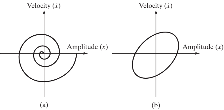
FIGURE 13.18 Attractor.
