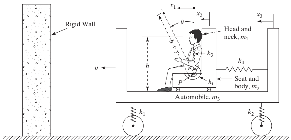
FIGURE 6.44 Modeling of an automobile hitting a rigid wall.
