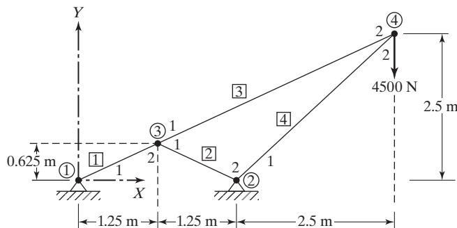
FIGURE 12.21 Crane.
