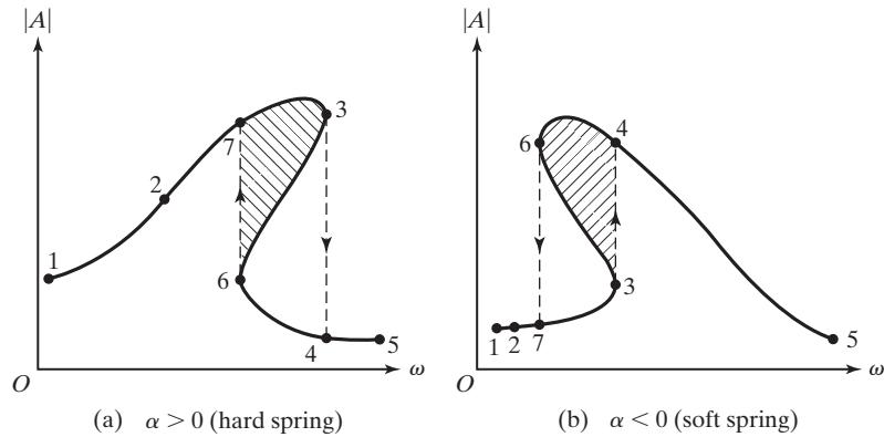
FIGURE 13.6 Jump phenomenon.
