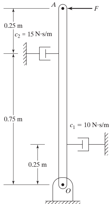
FIGURE 1.109 Rigid bar connected by dampers.
