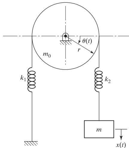
FIGURE 5.39 Mass hanging from a pulley.
