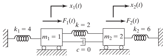
FIGURE 11.2 Two-degree-of-freedom system.
